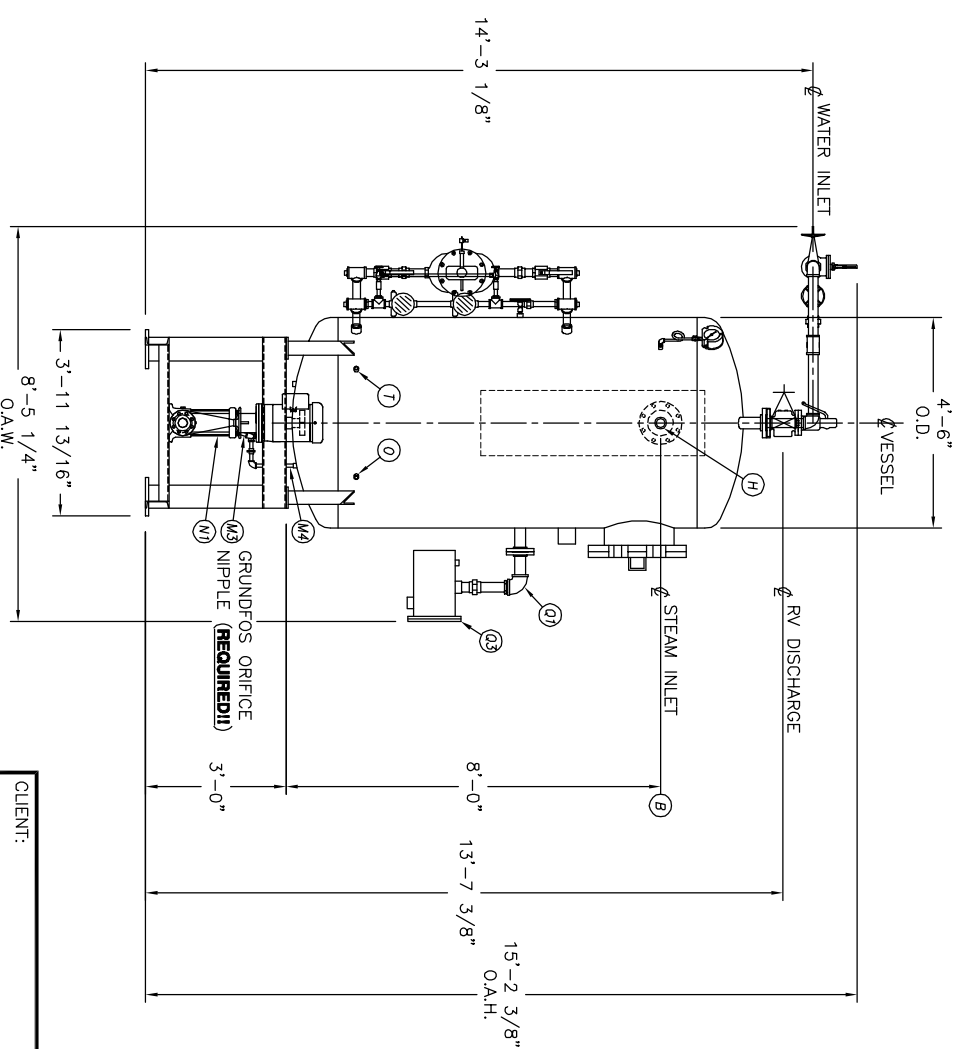
END VIEW
