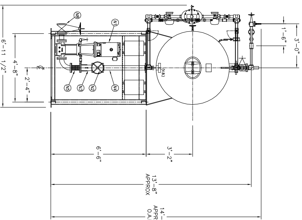
END VIEW
